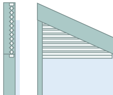
GABLE SLOPING HEAD BOX + SIDE BOX
