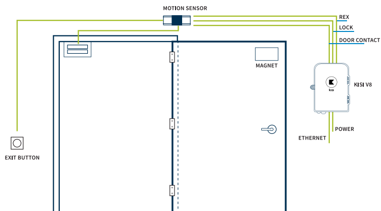
Wiring Diagram
